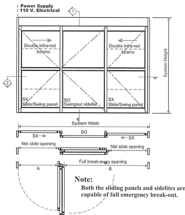
Elevation & floor plans Exterior view elevation
